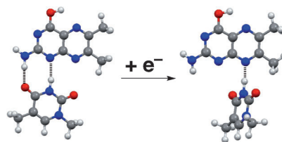
Figure 5. DFT-optimized structures of hydrogen-bonding adducts of Hdmp - -1-methylthymine at the B3LYP/6-31G(d) level of theory.
